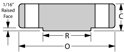
BLIND (BL)
