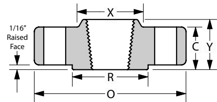
THREADED (TH)
